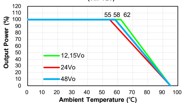
CHB200W12-72SXX-CMFD+HS(HD) Derating Curve (Vin=72V)
